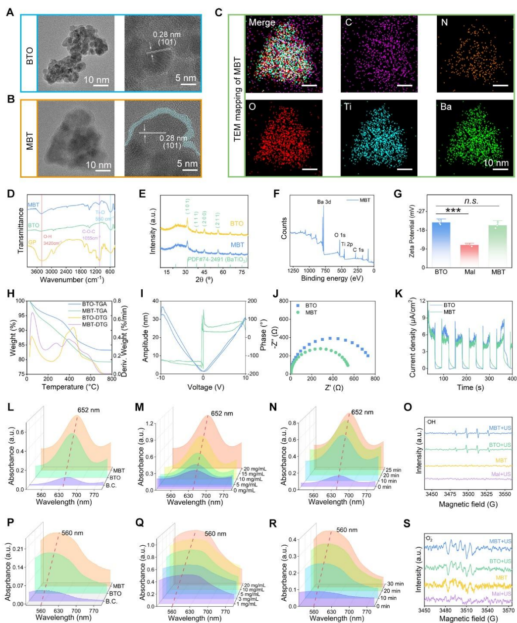
Figure 2. Piezocatalytic MBT nanosheets were fabricated for burst ROS generation. (A-B) TEM images of BTO and MBT. Scale bars: 10 nm and 5 nm; (C) TEM energy-dispersive mapping of MBT. Scale bar: 10 nm; (D) FT-IR spectrum; (E) XRD patterns; (F) XPS survey spectra; (G) Zeta potential (n = 3 biological replicates); (H) TG analysis; (I) PFM images; (J) EIS plots; (K) I-t curves; (L-N) UV-vis analysis for TMB assay; (O) EPR spectrum for detecting ·OH; (P-R) UV-vis analysis for NBT assay; (S) EPR spectrum for detecting ·O 2 - . All values are presented as mean ± SD. Statistical significance was assessed by one-way ANOVA. In inter-group comparisons,
