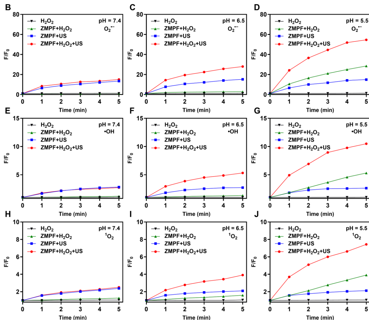
Figure 3. Evaluation of ZMPF-mediated ROS amplification through synergistic sonodynamic and chemodynamic activities. (A) Proposed ROS-generation mechanism involving ZMPF-mediated sonodynamic and chemodynamic activity. ROS generation of O 2 •- (B-D), •OH (E-G) and 1 O 2 (H-J) from H 2 O 2 , ZMPF+H 2 O 2 , ZMPF+US and ZMPF+H 2 O 2 +US groups in 10 mM PBS at pH 7.4, 6.5 or 5.5 (37 °C), respectively. F/F 0 represented the
