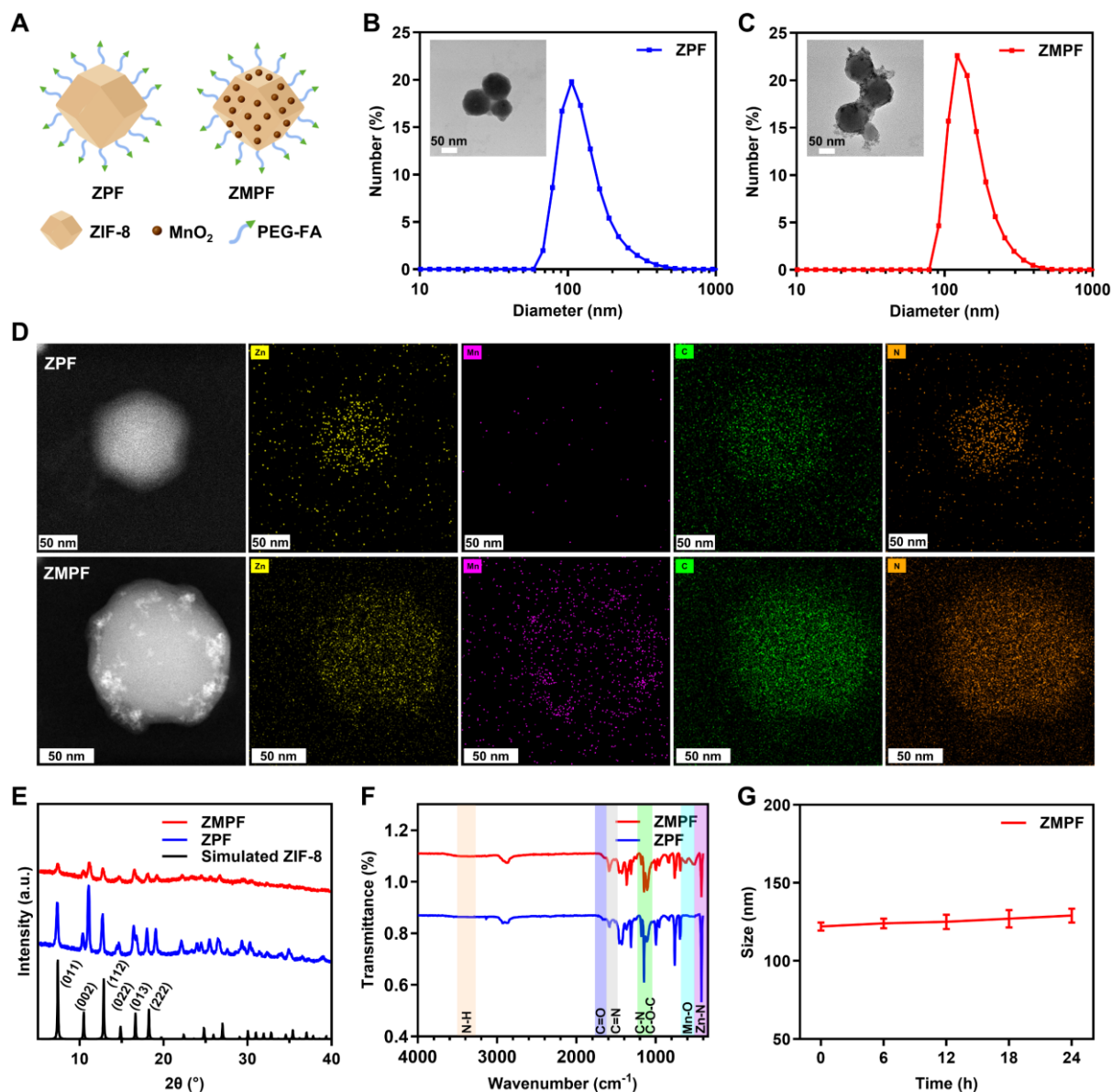
Figure 1. Fabrication and characterization of ZPF and ZMPF. (A) Schematic illustration of ZPF and ZMPF. DLS of ZPF (B) and ZMPF (C) with the corresponding TEM image as the inset (scale bar = 50 nm). Elemental mapping images (D), XRD patterns (E), and FTIR spectra (F) of ZPF and ZMPF. (G) Stability of ZMPF in deionized (DI) water evaluated by DLS at 0, 6, 12, 18 and 24 h (n = 3, mean ± s.d.).
