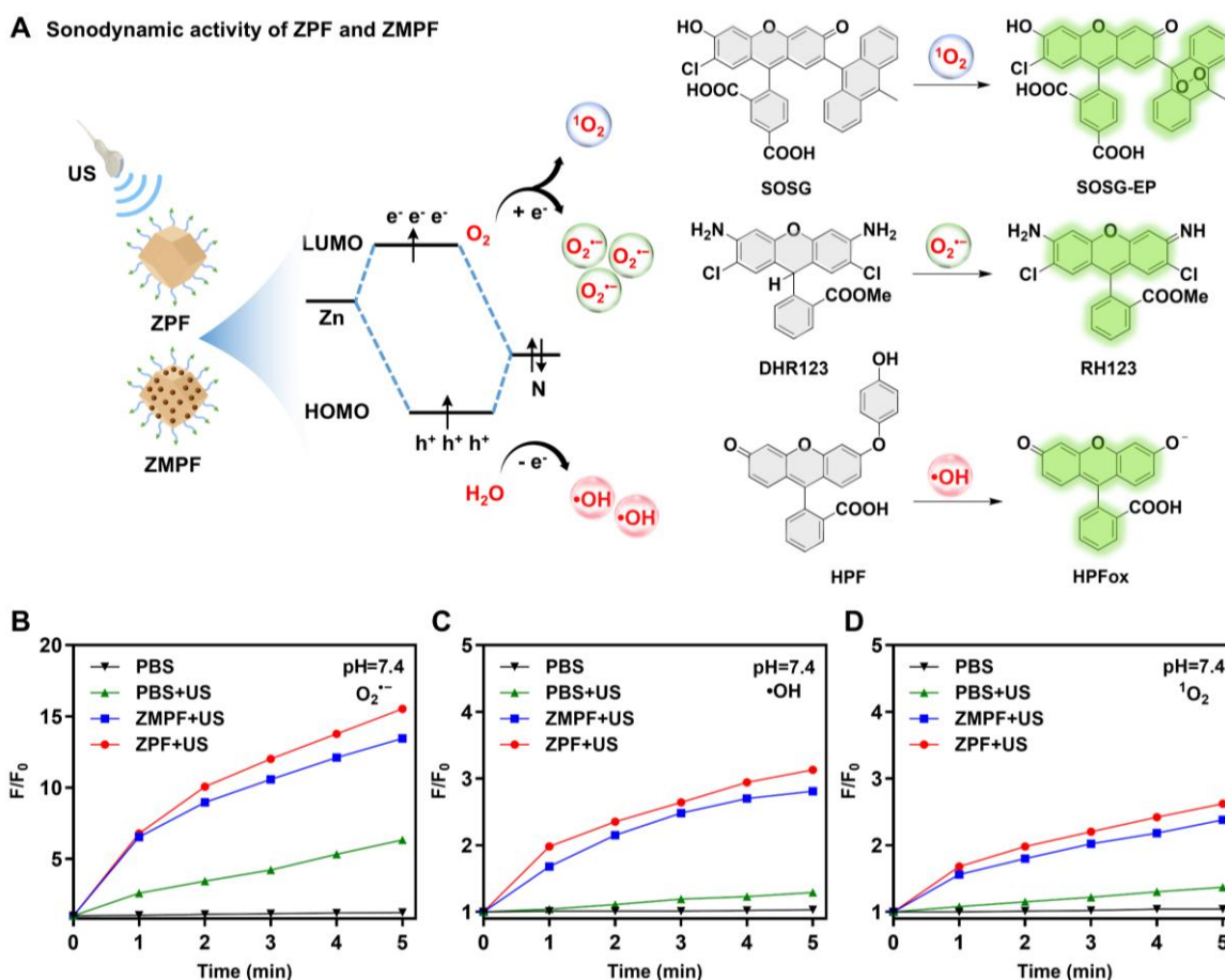
Figure 2. Evaluation of US-triggered sonodynamic ROS generation by ZPF and ZMPF.
