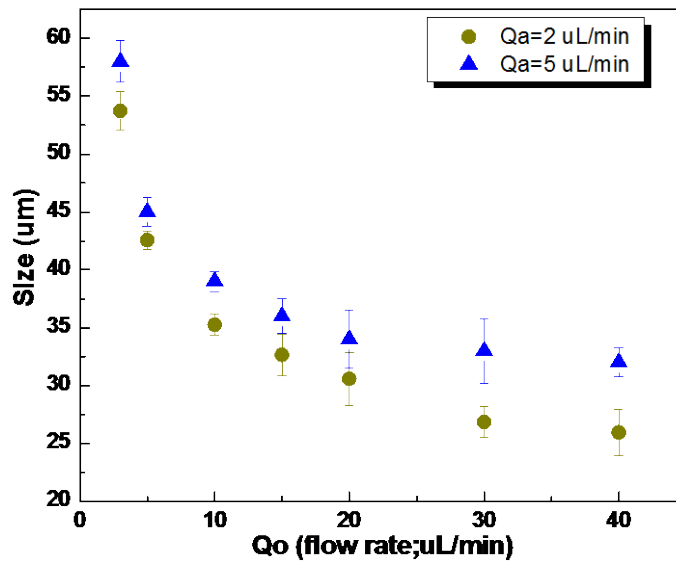
Fig. S1. Size variation in mean diameter of aqueous phase microspheres as a function of flow rate, Q_o=3\sim 40 ul/min and Q_a=2 and 5 ul/min.
